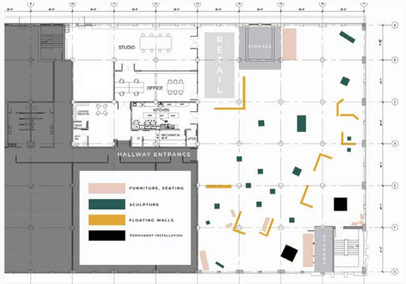
FLOOR PLAN
